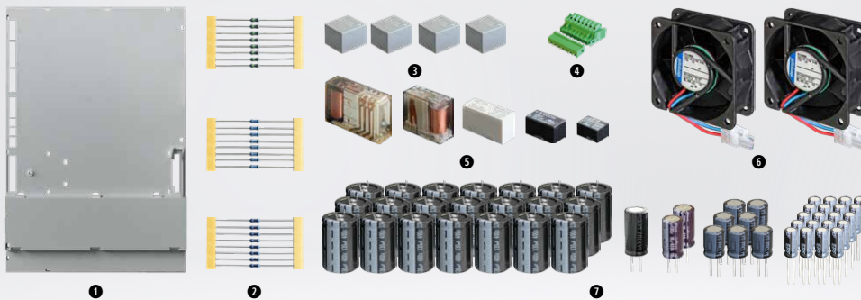
1. front panel 2. resistors 3. transformers 4. plug-in connections 5. relays 6. fan 7. electrolytic capacitors
